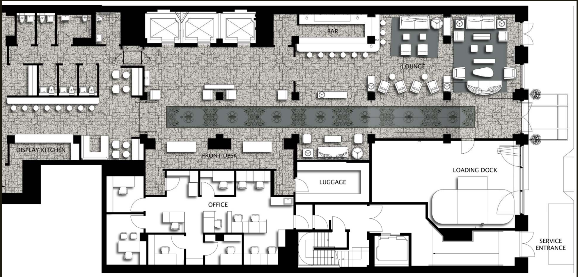
lobby & bar floor plan
